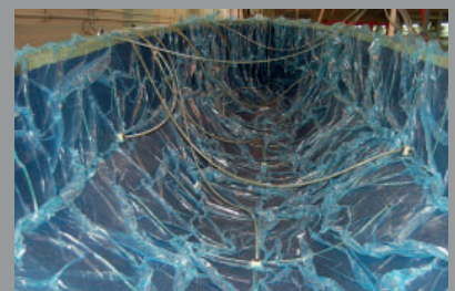
The Tricat 30 infusion-built central hull
